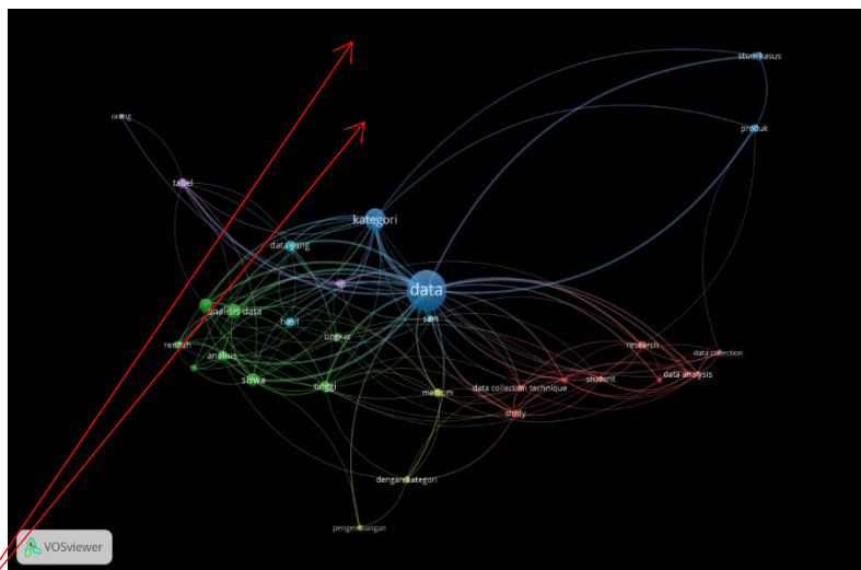
networking visualization
