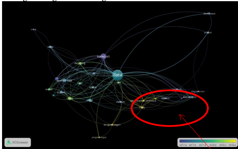
overlay visualization
