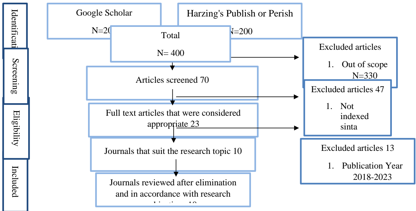
Figure 1. PRISMA Flowcharts
