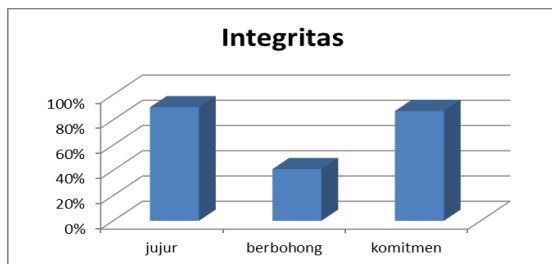
Gambar 3. Diagram Integritas
