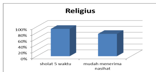
Gambar 2. Diagram Religius
