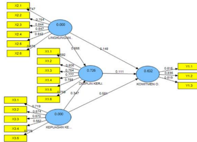
Gambar 1. Diagram Jalur Output PLS
